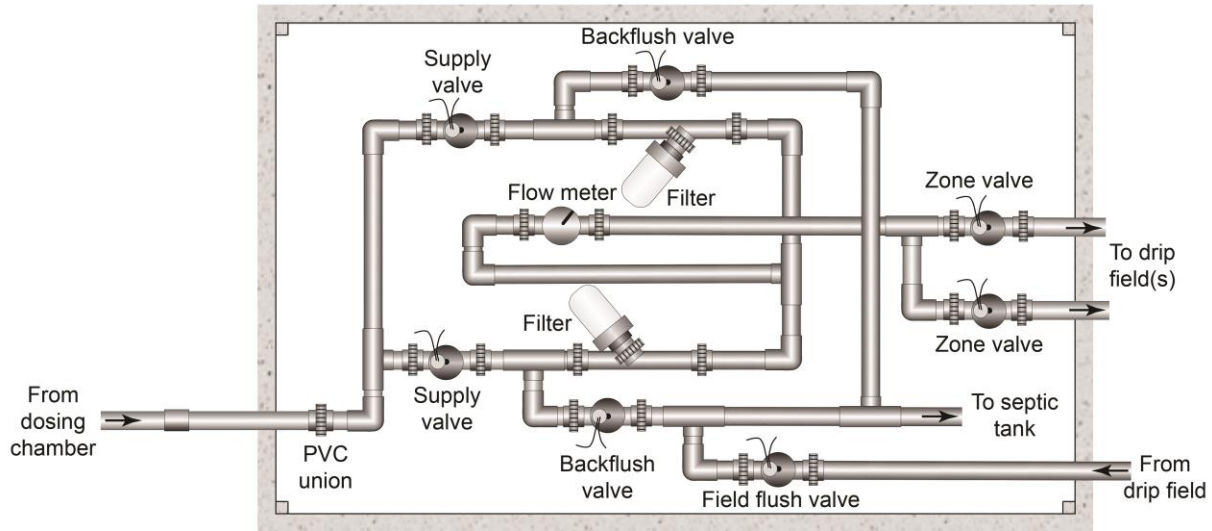
Figure 4-8. Overhead view of filter, valve, and meter assembly for a noncontinuous flush system.
