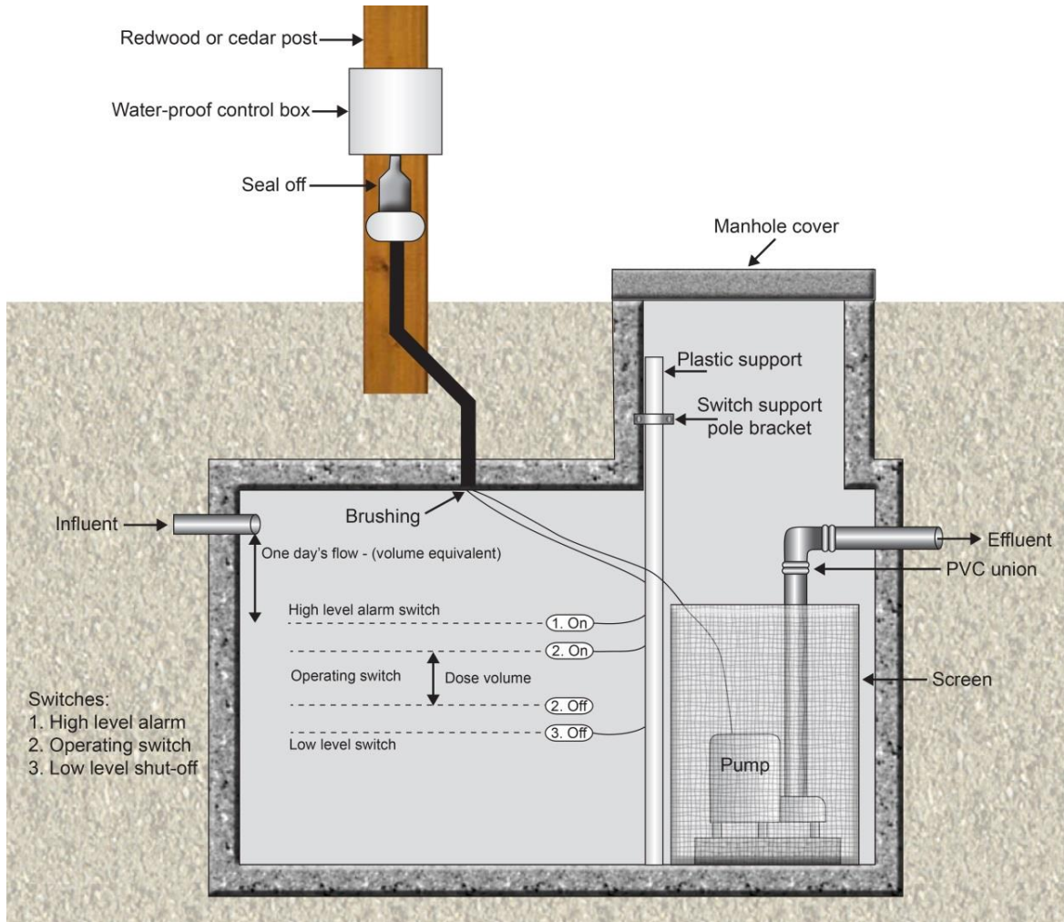
Figure 4-20. Dosing chamber with a pump and screen.
