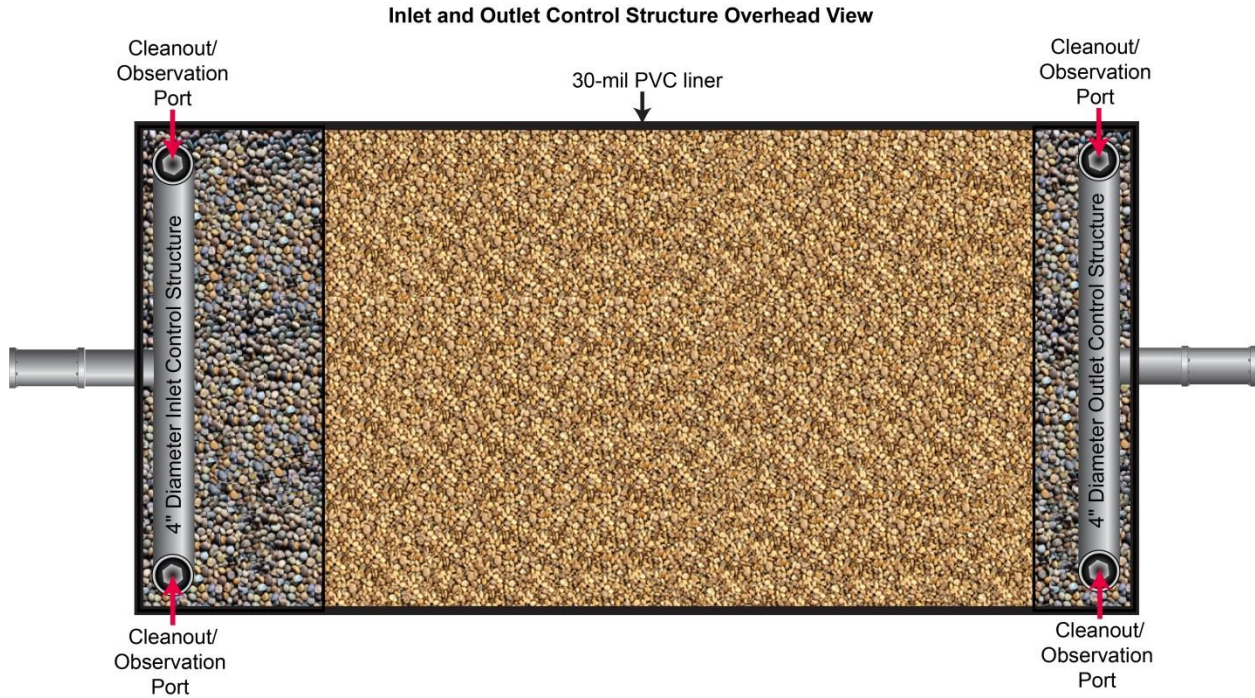
Figure 4-51. Overhead view of a wetland showing the inlet and outlet control structures in relation to the wetland width.
