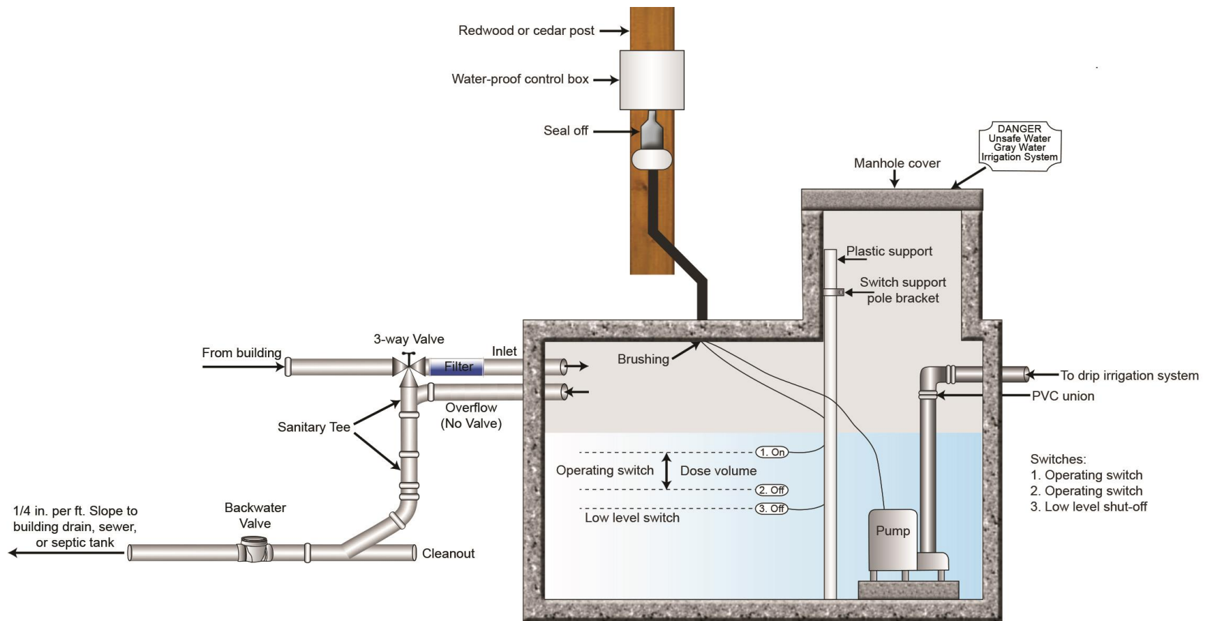
Figure 4-19. Gray water system (single-tank pumped).
