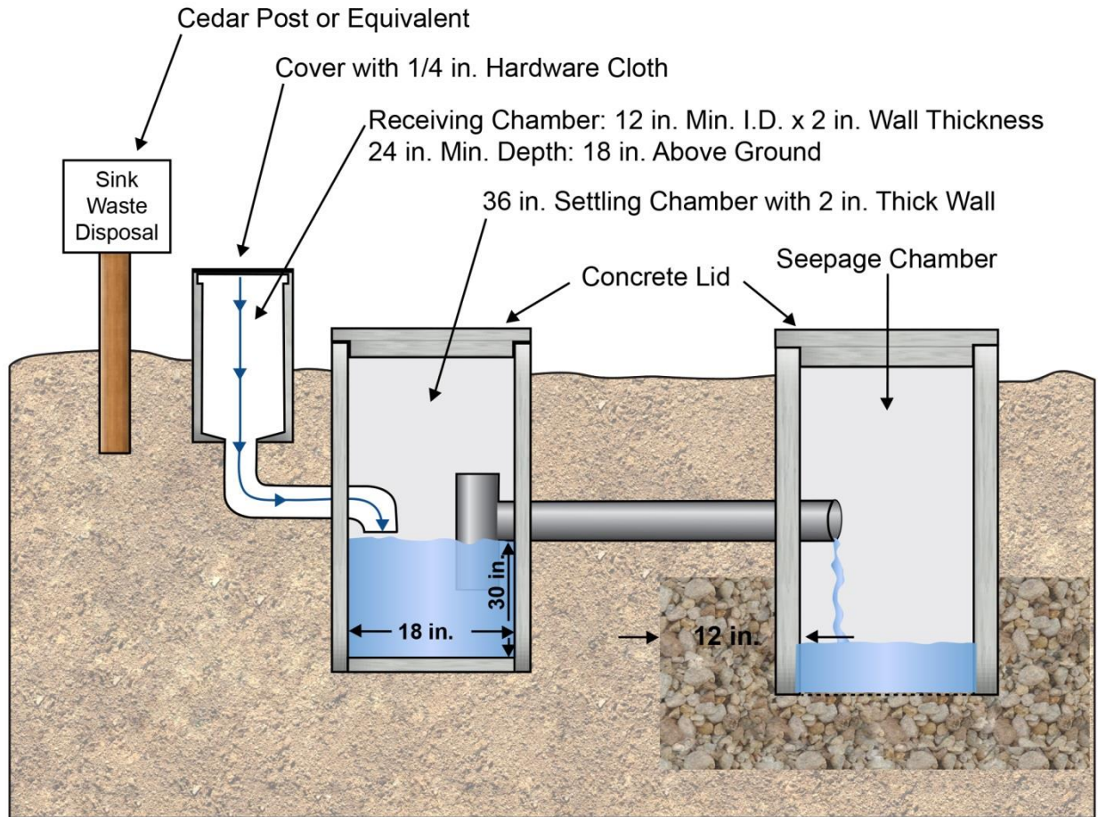
Figure 4-17. Cross section of gray water sump system.
