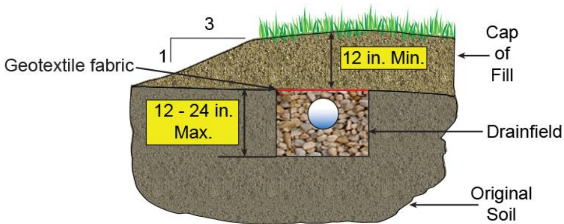
Figure 4-5. Cross-sectional view of a below-grade capping fill trench.
