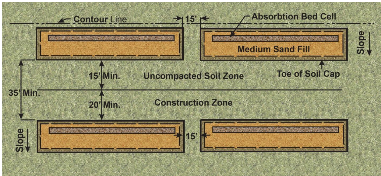
Figure 4-46. Mounds placed upslope and downslope of one another.
