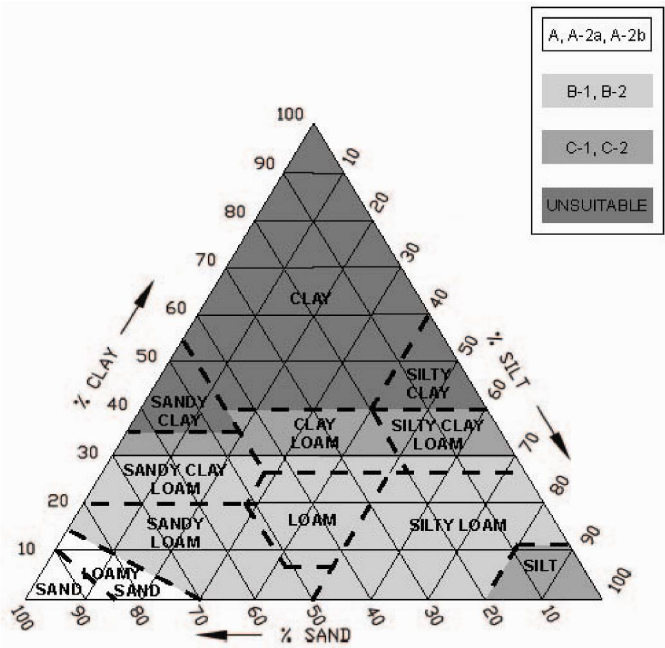
Soil texture determination triangle.
