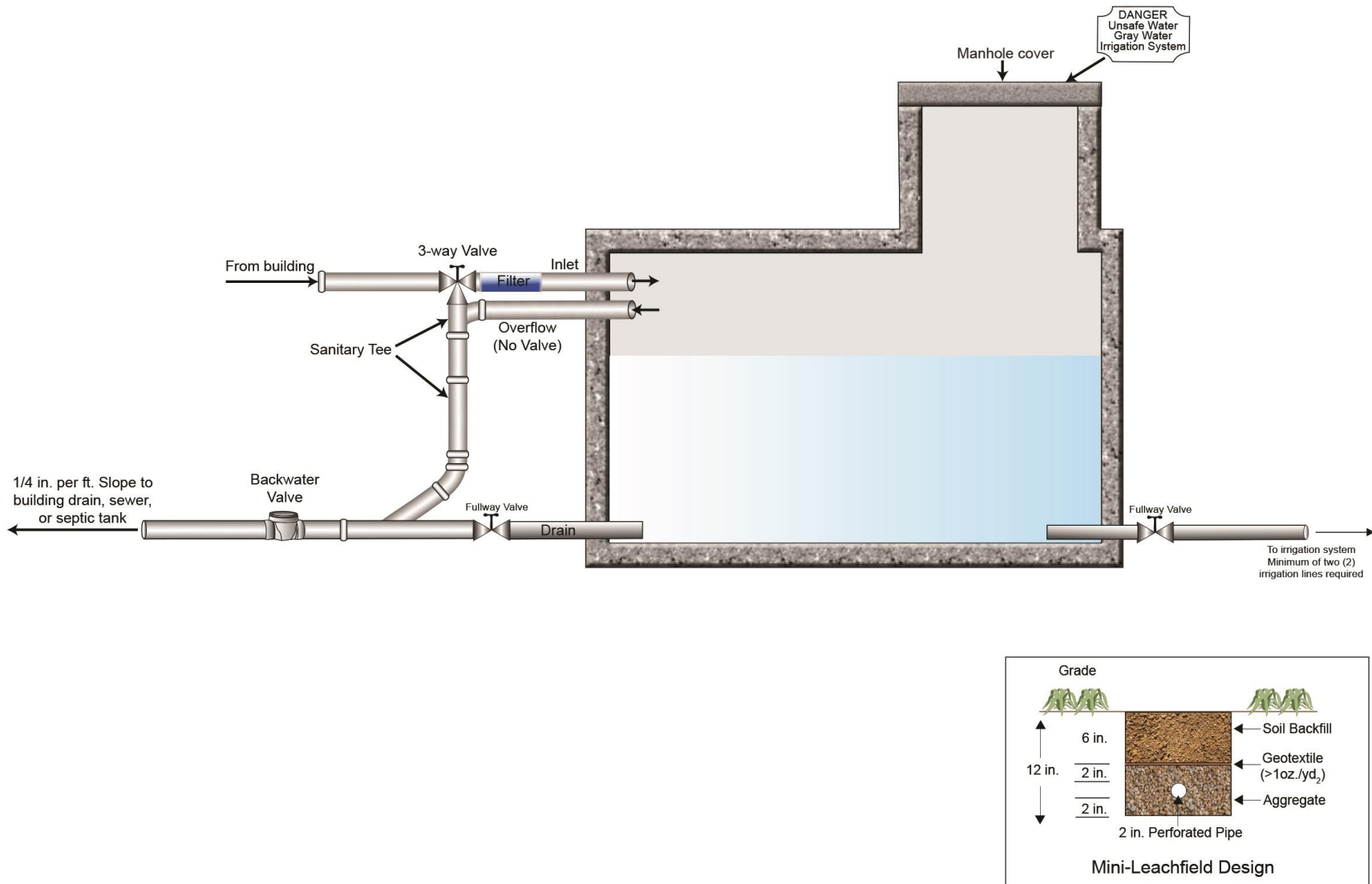
Figure 4-18. Gray water system (single-tank gravity).
