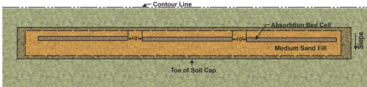
Figure 4-43. Multiple absorption bed cells installed in one sand mound.
